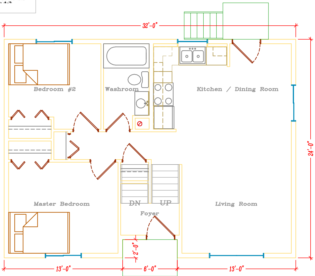
P1 Prelim Main Level 756 sq.ft.
