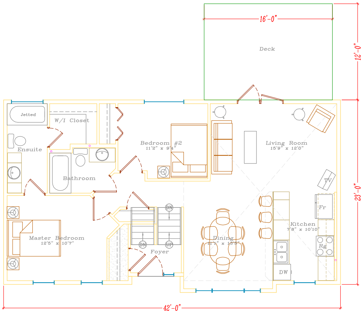
P1 Prelim Main Level 972 sq.ft.
