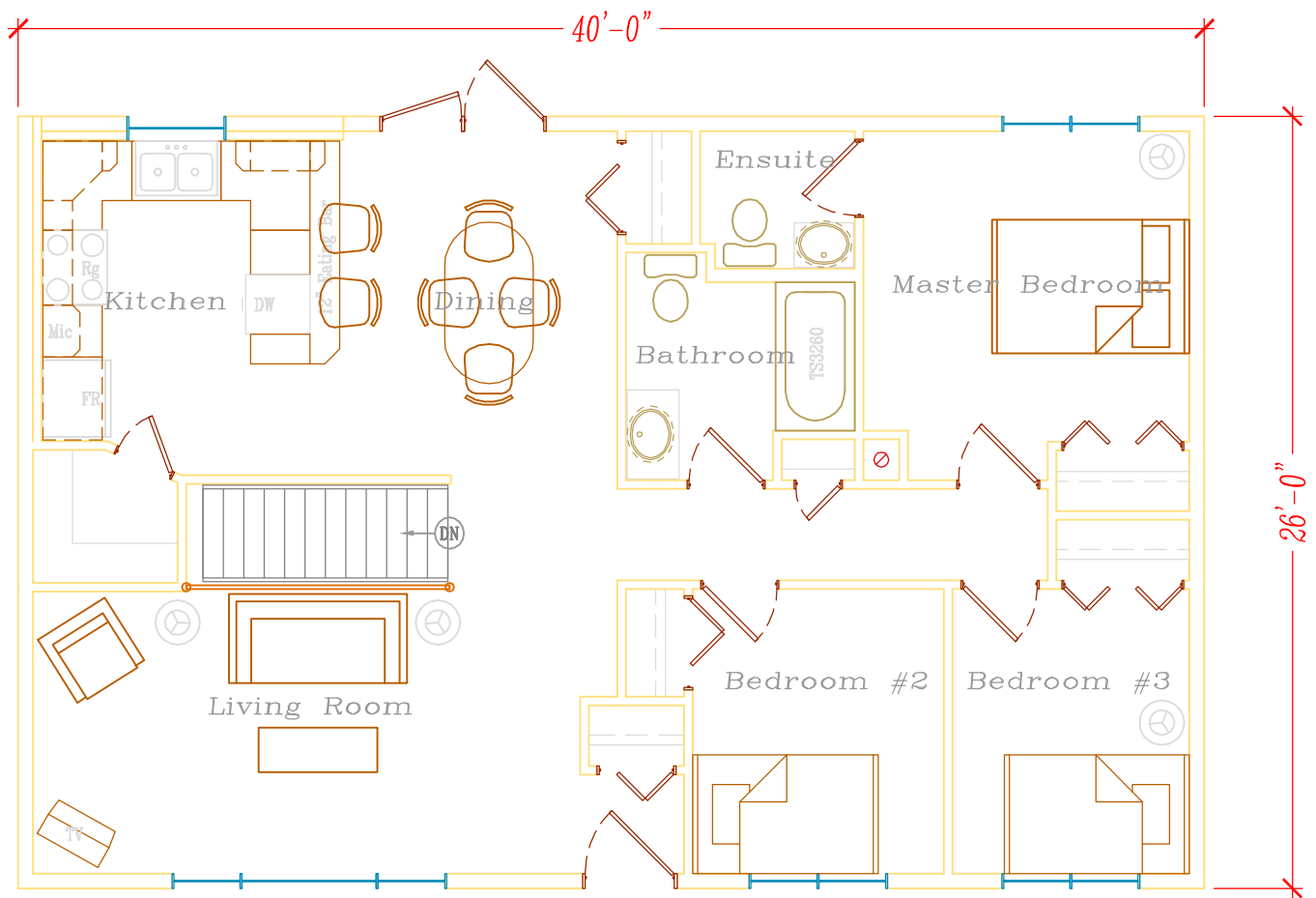
P1 Prelim Main Level 1040 sq.ft.
