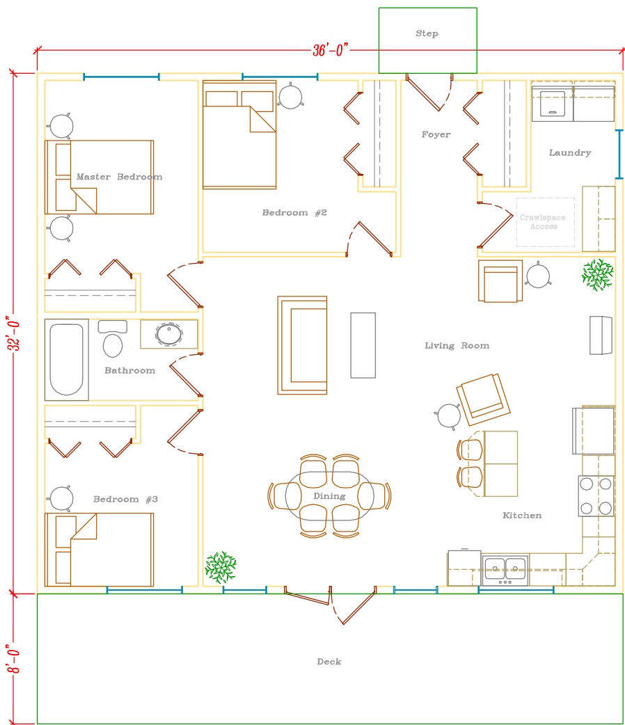
P1 Prelim Main Level 1152 sq.ft.
