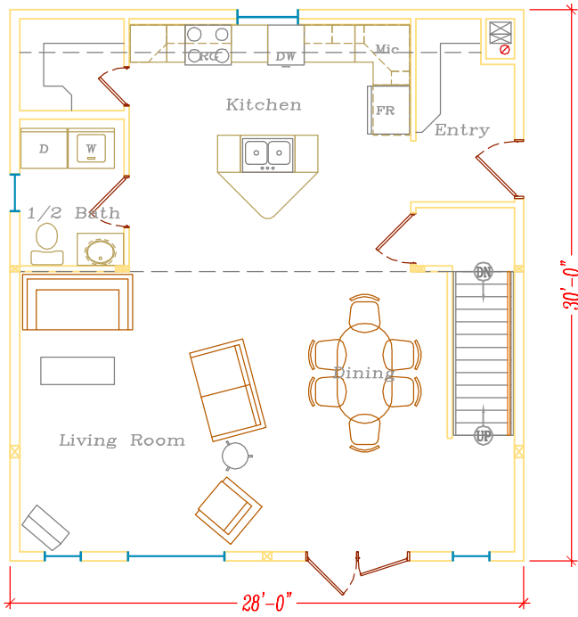
P2 Prelim 1st Level 840 sq.ft.
