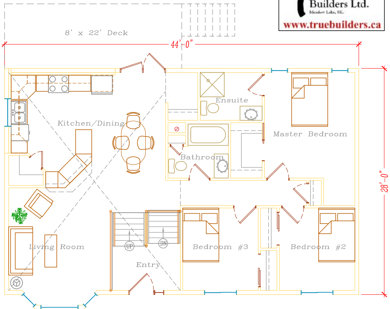
P1 Prelim Main Level 1246 sq.ft.
