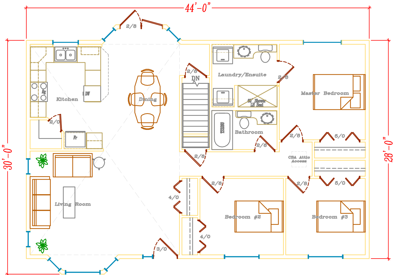
P1 Prelim Main Level 1284 sq.ft.
