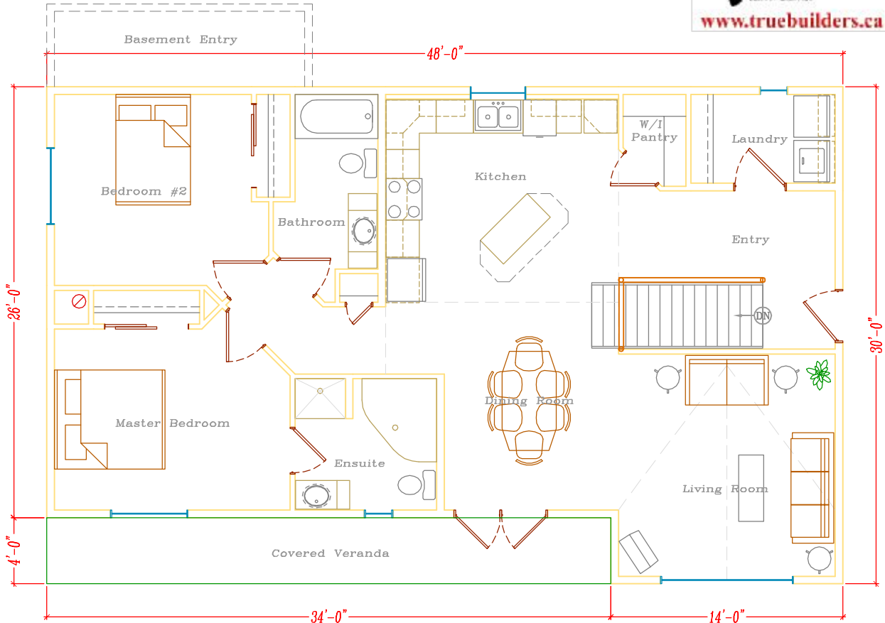
P1 Prelim Main Level 1304 sq.ft.
