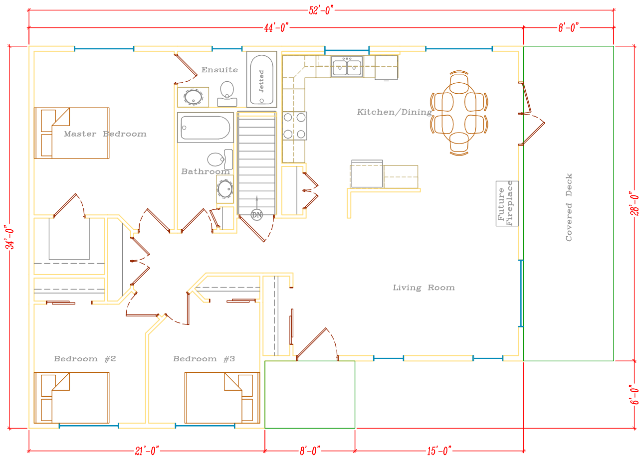
P1 Prelim Main Level 1358 sq.ft.
