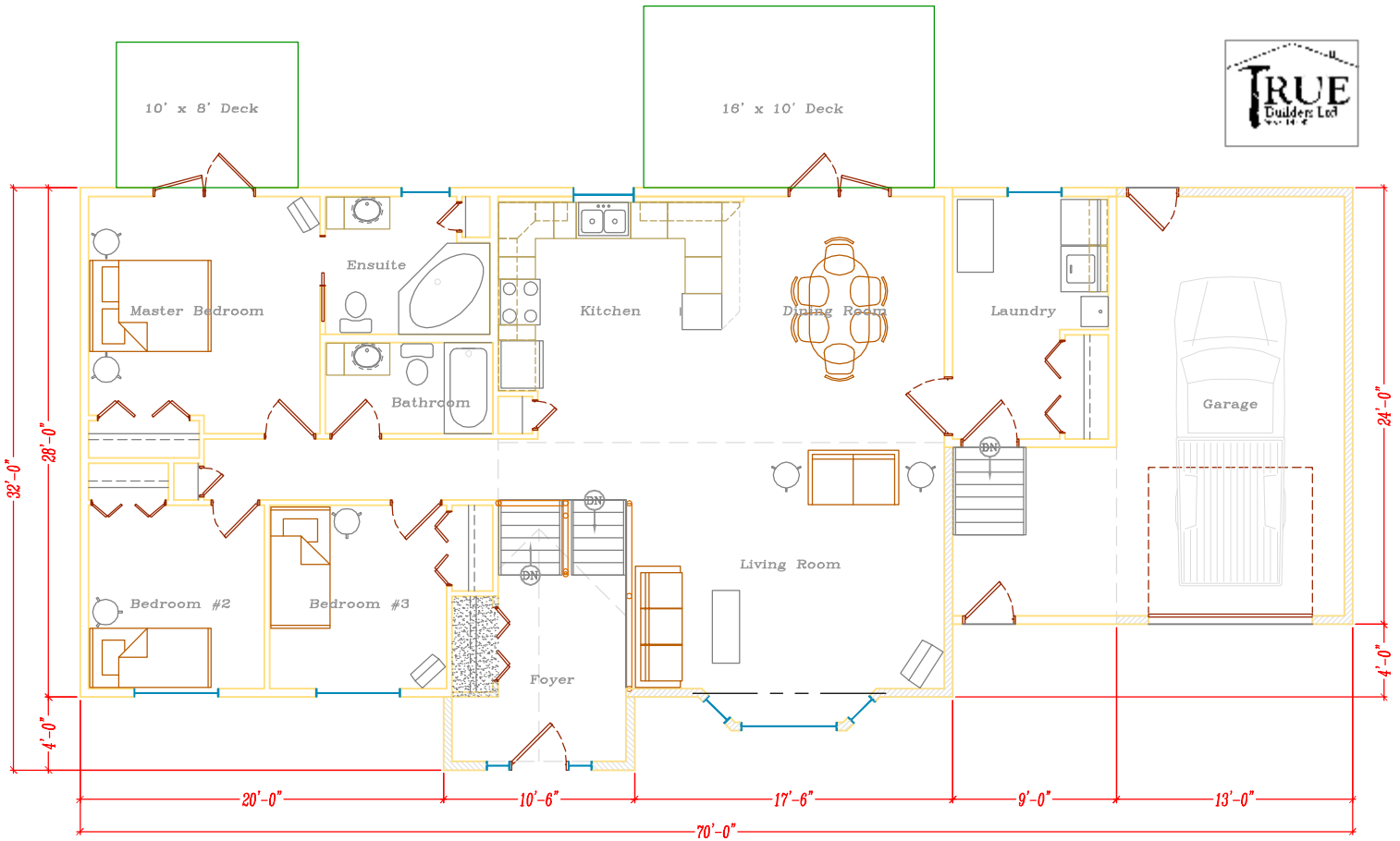
P1 Prelim Main Level 1629 sq.ft.
