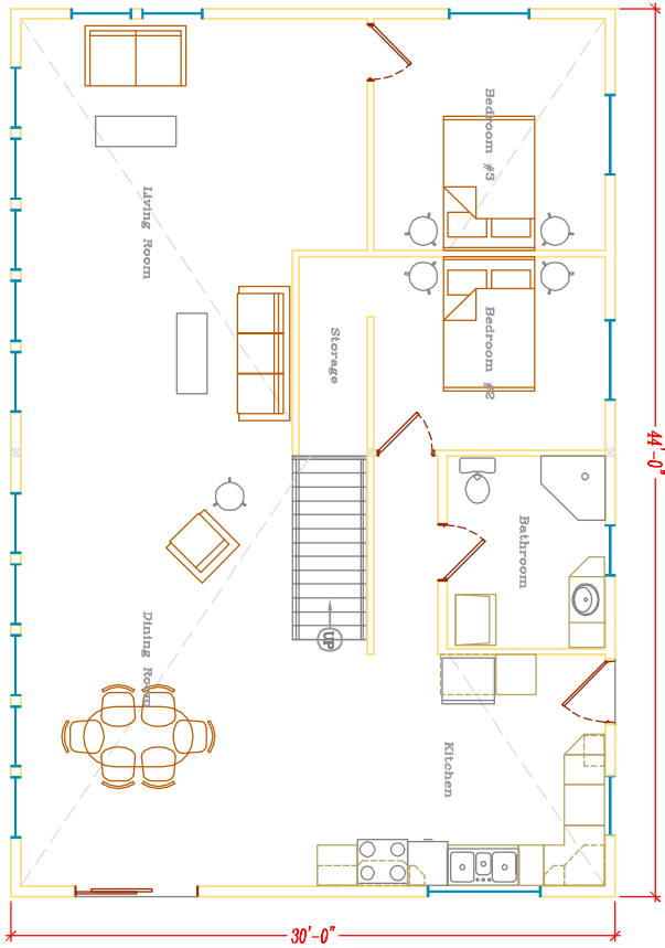
P1 Prelim Main Level 1380 sq.ft.
