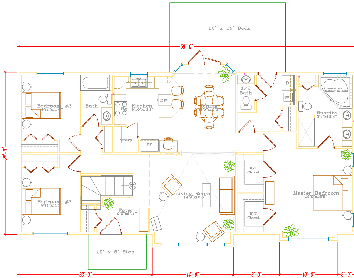
P1 Prelim Main Level 1679 sq.ft.
