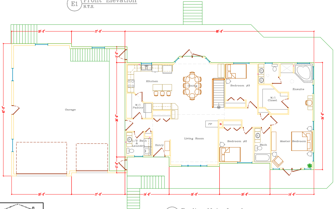
P1 Prelim Main Level 1956 sq.ft.
